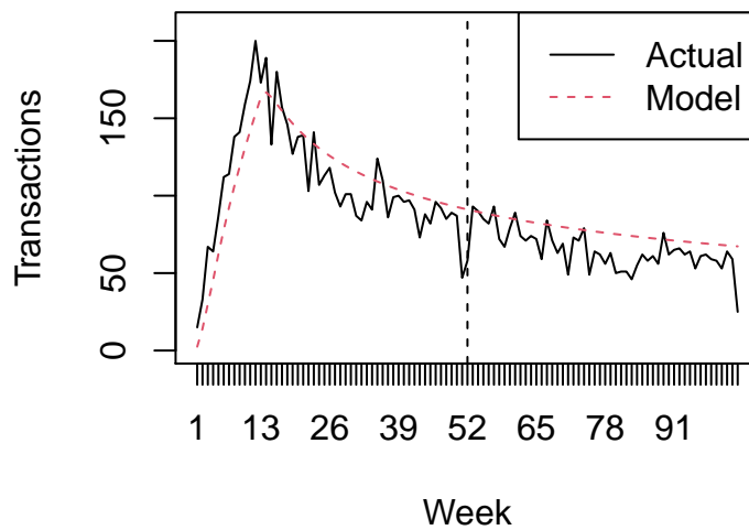
Figure 4: Weekly actuals vs. MBG/CNBD-k predictions
