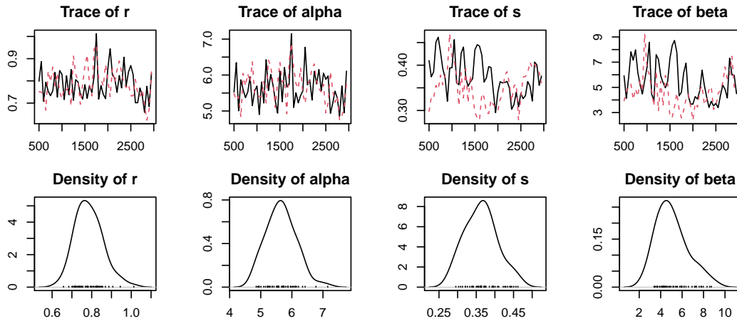
Figure 5: MCMC traces and parameter distributions of cohort-level parameters
