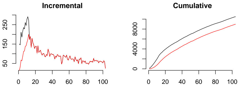
Figure 2: Weekly trends for the grocery dataset
