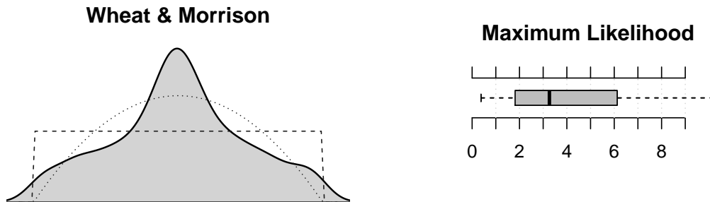
Figure 3: Diagnostic plots for estimating regularity
