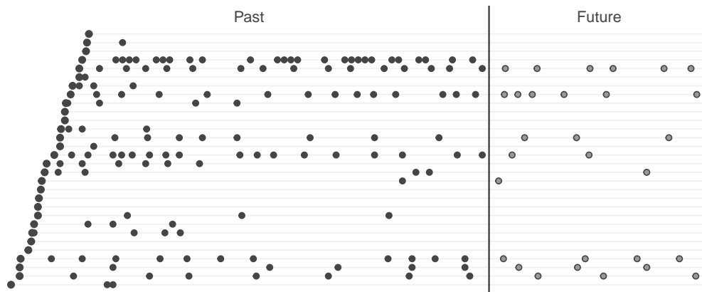
Figure 1: Timing patterns for sampled grocery customers
